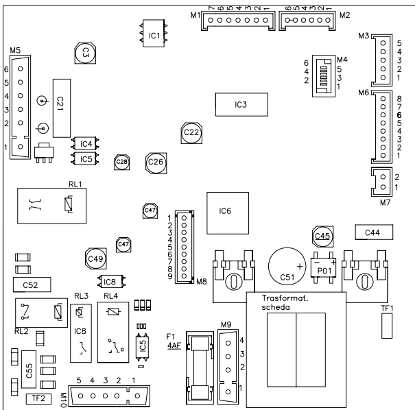
PRITED CIRCUIT BOARD - SM 20019 DIGITECH code 76677LA
