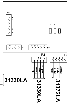
PRINTED CIRCUIT BOARD KOND DT - SK11003 code 76702LA
