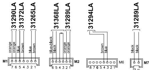
PRITED CIRCUIT BOARD - SM 20019 DIGITECH code 76677LA
